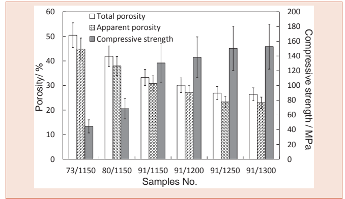
Figure 5: Total porosity, apparent porosity and compressive strength of the intermediate porous sintered blocks.
