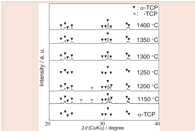
Figure 3: XRD patterns of starting powder \alpha -TCP and samples after sintering between 1150 and 1400 °C.
