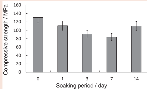
Figure 8: Compressive strength variation of 91/1150 samples before and after soaking for 1, 3, 7 and 14 d, respectively.
