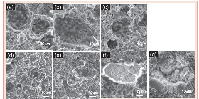
Figure 6: Cross-section SEM images of the sintered intermediate porous blocks. (a) 73/1150, (b) 82/1150, (c) 91/1150. (d), (e), (f) and (g) are cross-section SEM images of 91/1150 samples after soaking for 1, 3, 7 and 14 d, respectively.
