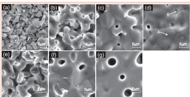
Figure 4: SEM images of green blocks (a) and dense sintered blocks. Surface: (b) 1150 °C, (c) 1300 C, (d) 1400 °C. Cross-section: (e) 1150 °C, (f) 1300 °C, (g) 1400 C.
