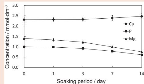
Figure 10: Concentrations of Ca, P and Mg in SBF solution after soaking 91/1150 samples for 1, 3, 7 and 14 d, respectively.
