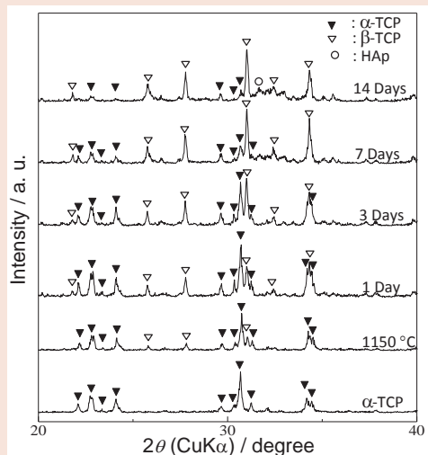
Figure 9: Crystalline phases changes of 91/1150 samples before and after soaking for 1, 3, 7 and 14 d, respectively.
