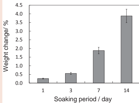
Figure 7: Weight changes of 91/1150 samples after soaking for 1, 3, 7 and 14 d, respectively.
